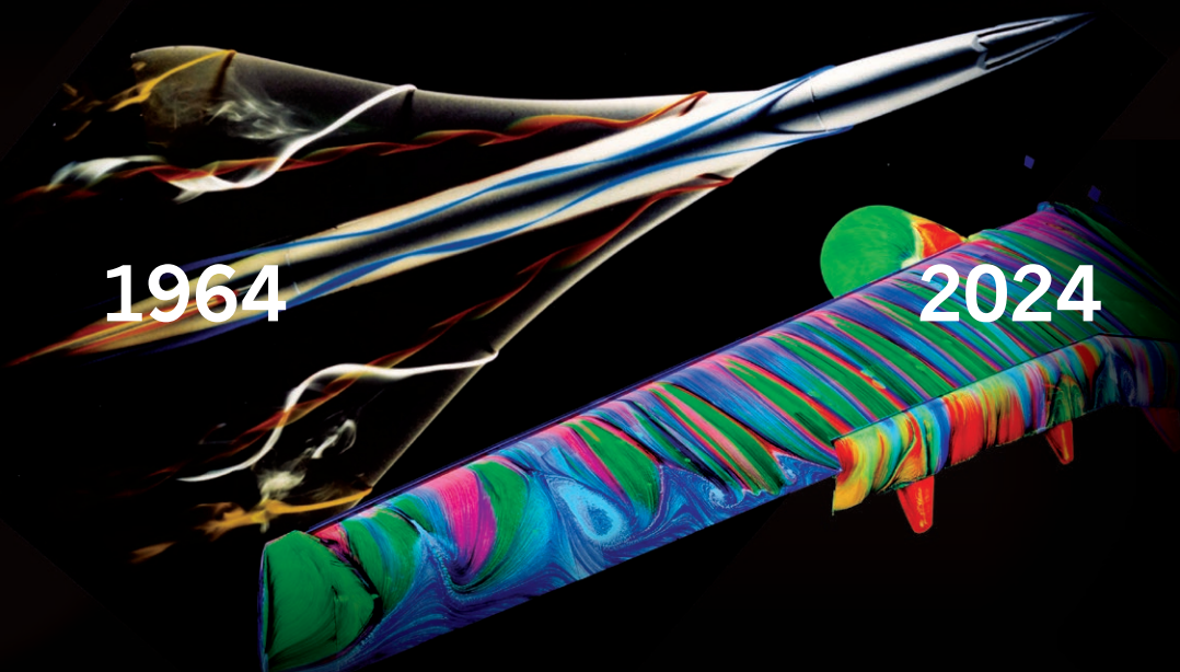
Visualization of leading edge vortices shedding of Concorde Credit Henri Werlé
