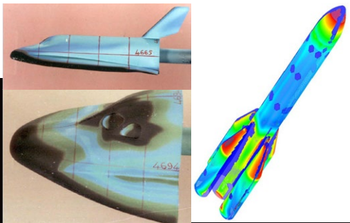
SURFACE MEASUREMENT TECHNIQUES OF WALL HEAT FLUX. Blowdown hypersonic wind tunnels at ONERA (Meudon) – Credit ONERA
